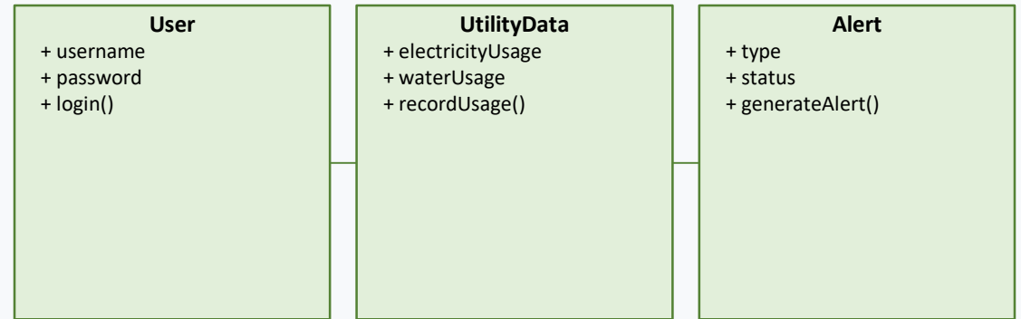
Class Diagram
