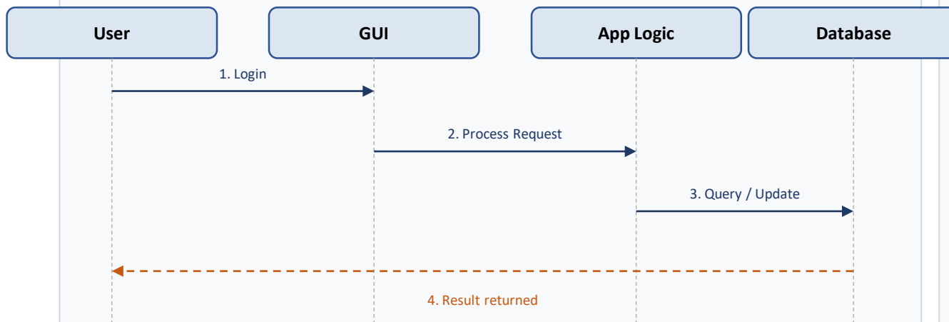
Sequence Diagram
